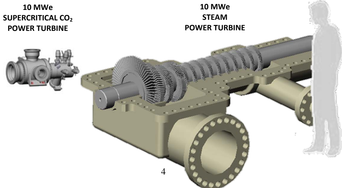
Figure 3: Echogen’s 10 MWe sCO 2 power turbine compared to a 10 MWe steam turbine.
