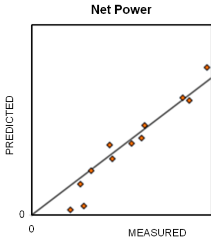
Figure 12: Measured vs. predicted net power output for the 250 kWe demonstration heat engine at AEP.
