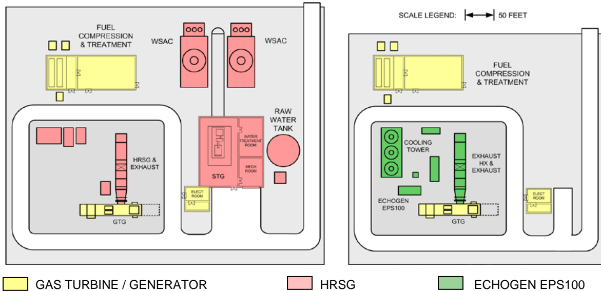
Figure 6: The Echogen EPS100 heat engine requires a smaller installation footprint compared to a heat recovery steam system for gas turbine heat recovery.
