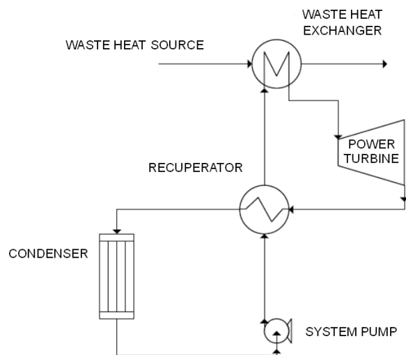
Figure 1: Simplified process flow diagram for the Echogen heat engine.
