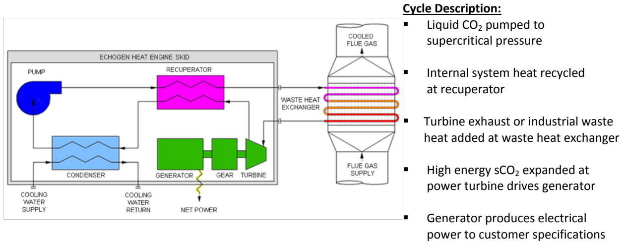
Figure 2: The Echogen Cycle is a compact, high-efficiency solution for exhaust heat to power from large scale industrial and utility applications including concentrating solar power.
