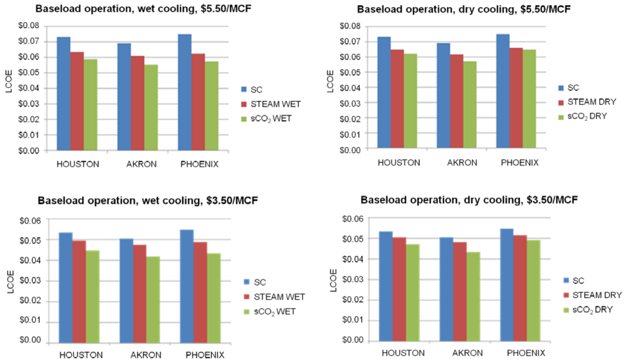
Figure 8: Baseload operation using an Echogen EPS100 for bottom cycling results in a 10 to 20 percent LCOE improvement compared to a simple cycle GT or CCGT with a steam bottoming cycle under wet-cooled conditions, and 4 to 15 percent LCOE improvement for dry-cooled cases.
