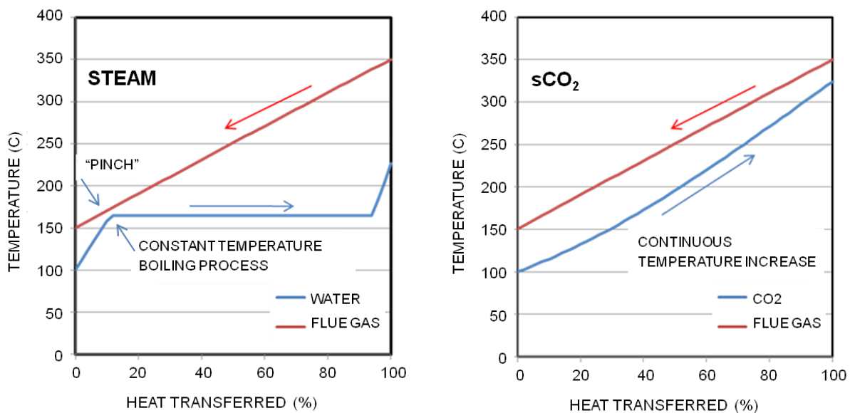
Figure 4: Unlike steam (left), supercritical CO 2 (right) is a single-phase fluid during heating in the exhaust heat exchanger resulting in higher fluid temperatures and cycle efficiencies.
