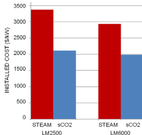
Figure 7: Installed cost per kilowatt for Echogen EPS100 is up to 40% less compared to heat recovery steam.
