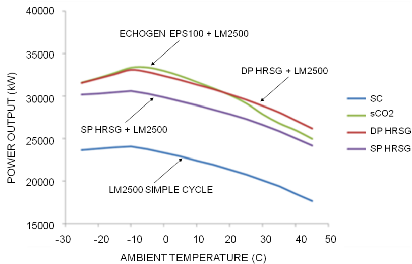
Figure 5: Power out versus ambient temperature -- Echogen’s EPS100 heat engine performance is comparable to a double-pressure heat recovery steam system. The simple cycle LM2500 gas turbine (SC) is shown for reference.
